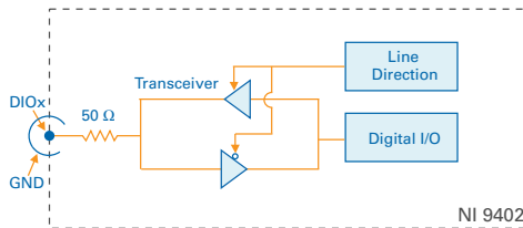
Figure 1. NI 9402 Circuitry for One Channel
